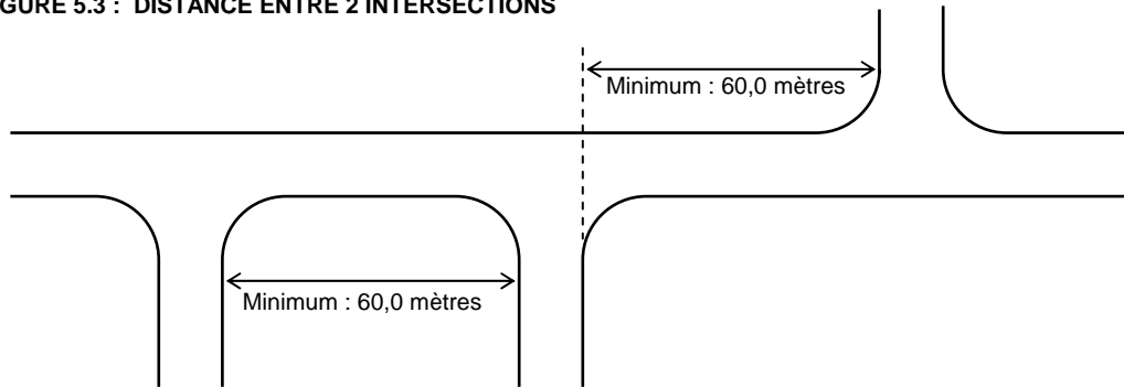
FIGURE 5.3 : DISTANCE ENTRE 2 INTERSECTIONS
